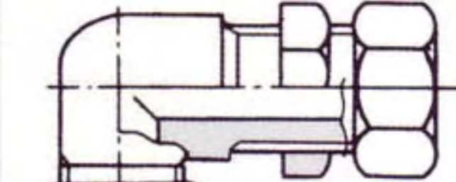
HE :隔壁締付エルボ
